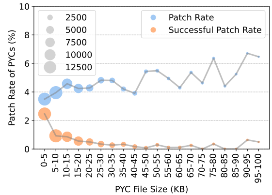
Figure 12: In the wild, file size strongly impacts patch success rates, but does not strongly impact patch attempt rates.
