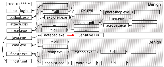
Fig. 2: Dependency graph of the motivating attack
