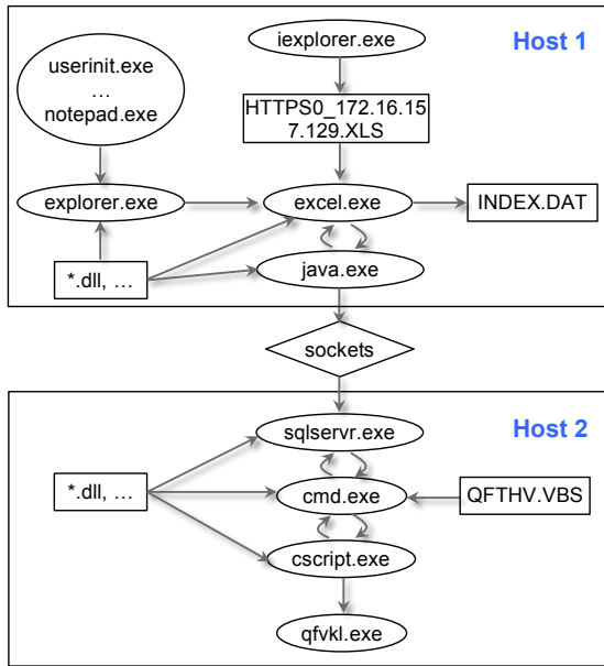
Fig. 5: Dependency graph of case 2 - Malicious Excel Macro
